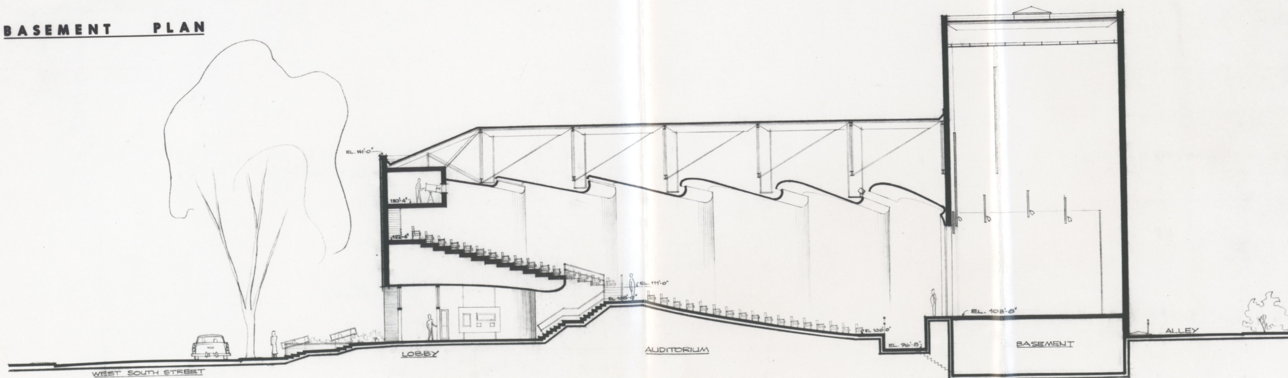
SECTION thru UNIT 'A'
