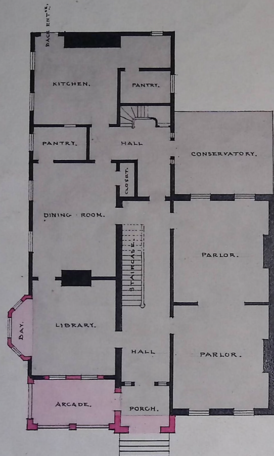
PRINCIPAL FLOOR.
