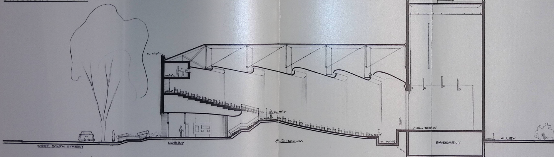
SECTION thru UNIT 'A'
